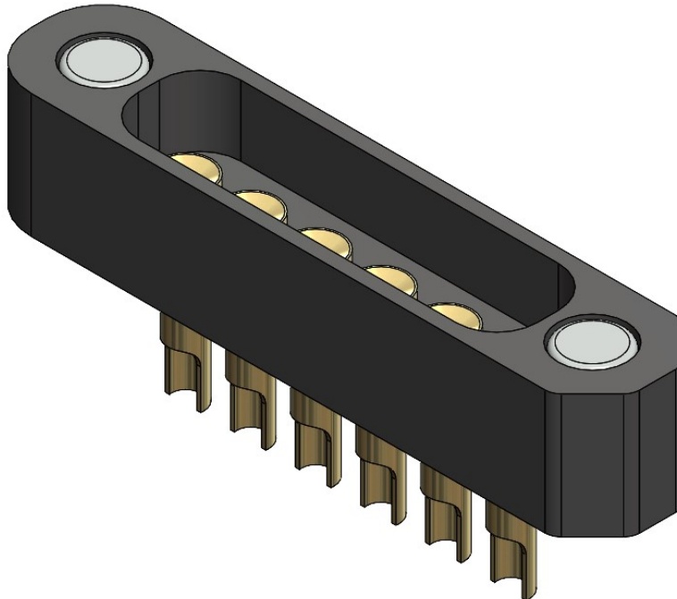
Figure 1: Illustration of chamfer to indicate polarization.
